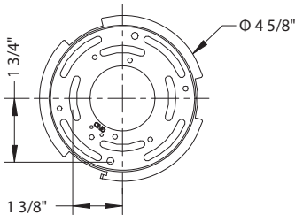
CEILING PLATE
