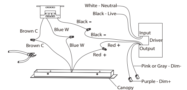
Fig. 4 Driver Wires
