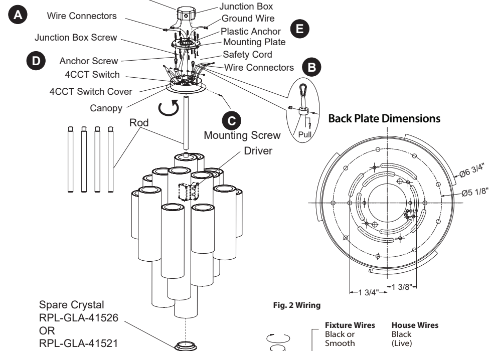
Fig. 1 U.L. Approved 200LB. MAX Outlet Box and Hardware (Sold Separately)
