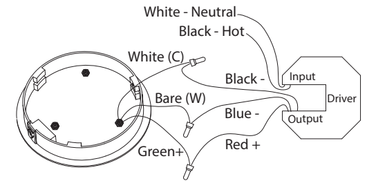
Fig. 3 Wire Diagram
