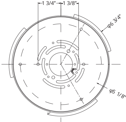
Backplate Dimensions
