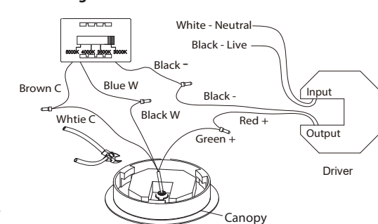
Fig. 4 Driver Wires
