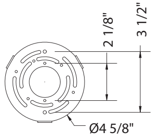
Mounting Plate
