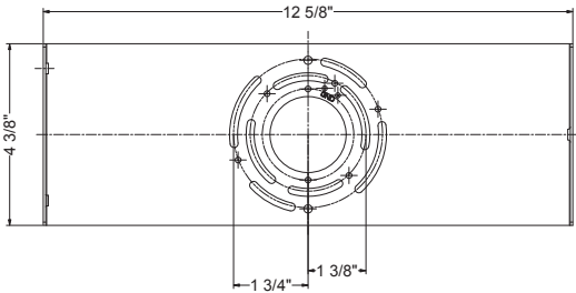
Back Plate Dimensions
