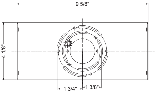
Back Plate Dimensions
