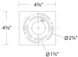
Mounting Plate
